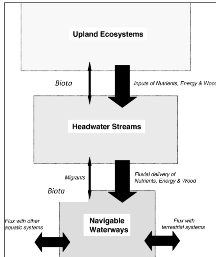
Figure 3. Natural connectivity model between uplands, headwater streams and larger streams and rivers
