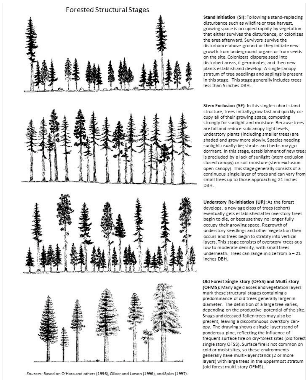
Figure 4. Description of forest structural stages used to classify vegetation for the Malheur National Forest plan revision (Justice and Countryman 2006)
